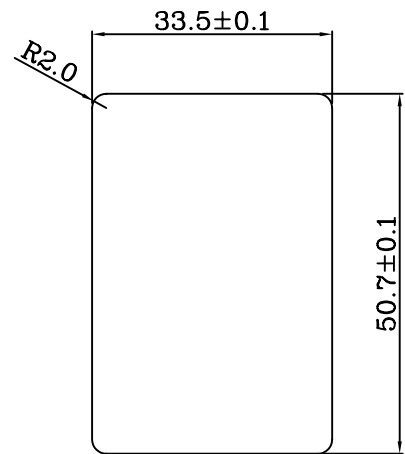
PANEL CUT-OUT
