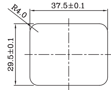
PANEL CUT-OUT
