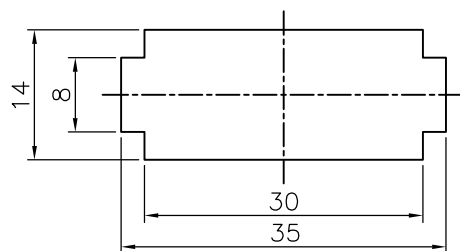
PANEL HOLE
