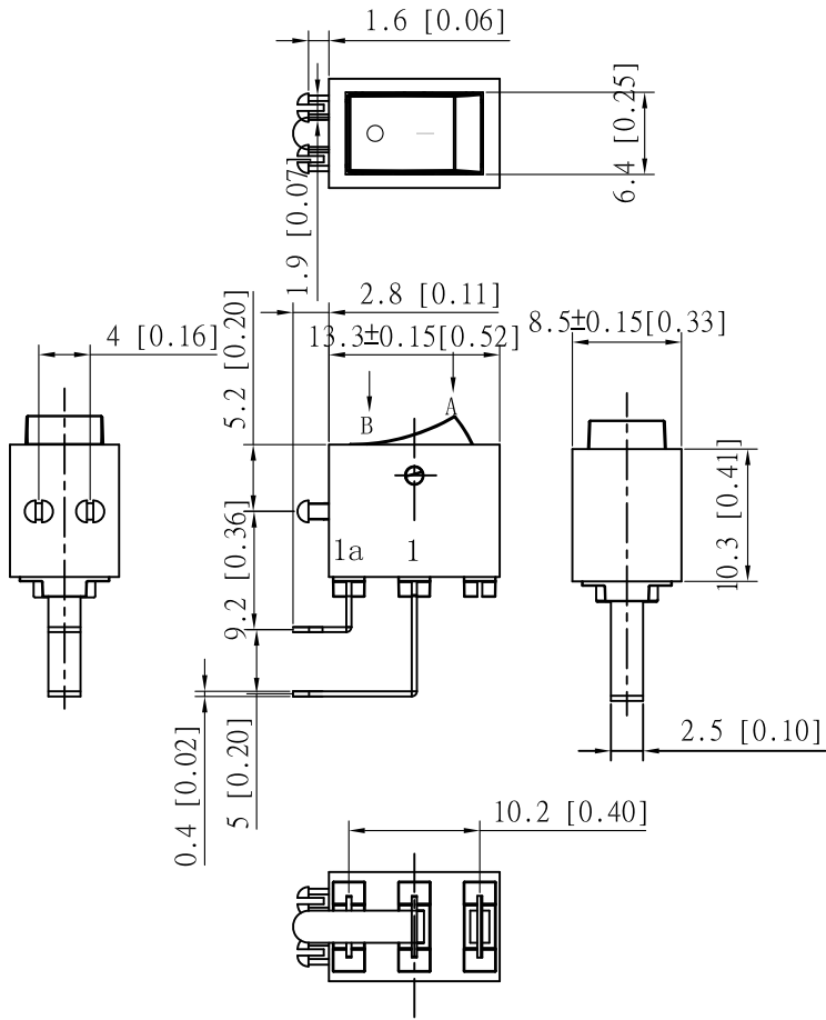
P.C MOUNTING
