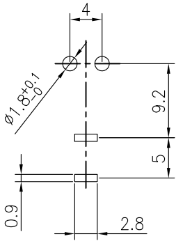
P.C MOUNTING
