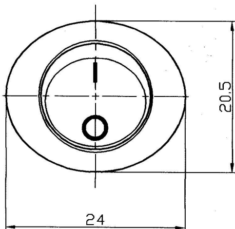
Small Rocker Switch R13-234 Series
