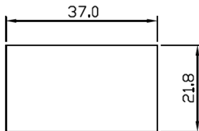
Panel Cutout
