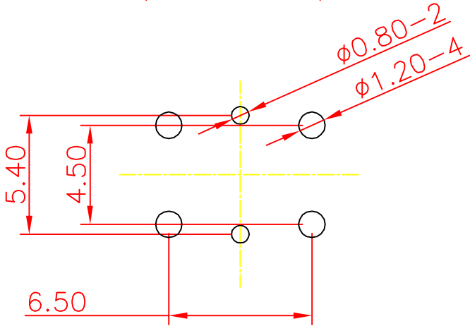
Mounting pattern
